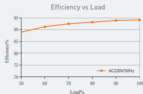
YSD-200WUF-24
