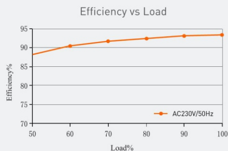
YSD-200WUF-12
